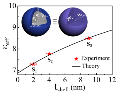
FIG. 5. Increase of the permittivity with increasing thickness of the graphite shell. The solid line represents a fit to the experimental data (red star with error bar) based on the Bruggeman theory. The inset shows the uniform structure that mimics the Ni/C nanocapsule core/shell structure.
