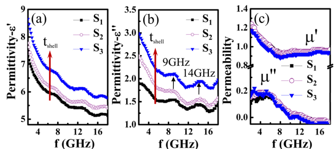
FIG. 4. Permittivity \epsilon and permeability \mu of the samples S_1 , S_2 , and S_3 . (a) and (b) Frequency dependence of the real and imaginary parts of \epsilon and (c) frequency dependence of the real and imaginary parts of \mu .
