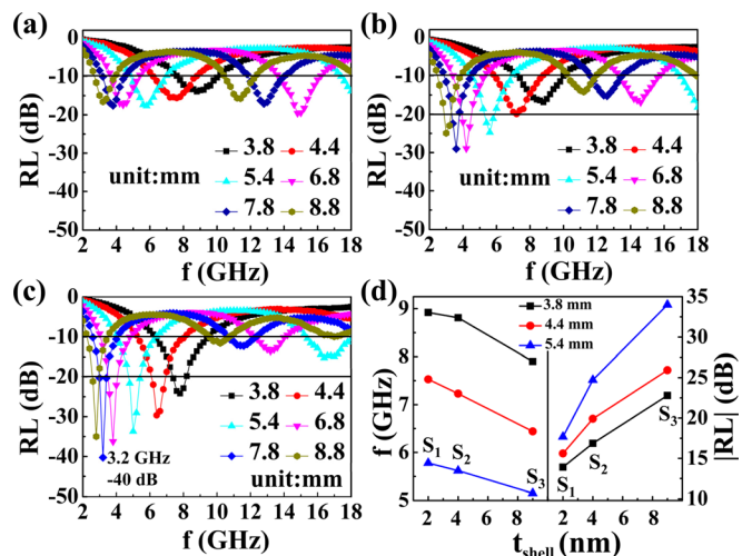
FIG. 3. (a)–(c) Frequency dependence of RL of S_1 , S_2 , and S_3 for different values of the thickness d of the absorbing layer and (d) comparison of the match frequency and RL values of S_1 , S_2 , and S_3 at different d values.
