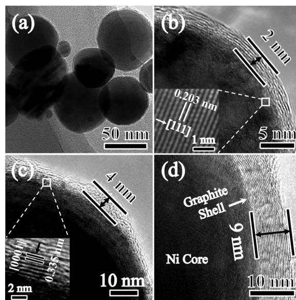
FIG. 1. Microstructure of Ni/C nanocapsules. (a) TEM image of sample S 1 and (b)–(d) HRTEM images of samples S 1 , S 2 , and S 3 with graphite shell thicknesses of 2 nm, 4 nm, and 9 nm, respectively. The insets of (b) and (c) show HRTEM images of the Ni core and the graphite shell.
