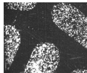
Fig. 3. Optical microscope image of patterned layer of NPC on glass support. Image size is 0.4 \times 0.4 \text{ mm}^2 .
